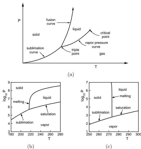
Figure 7.3: (a) Sketch of a typical phase diagram of a simple substance. The phase diagram shows the boundaries or coexistence curves between the solid, liquid, and gas phases. All three phases coexist at the triple point. For temperature and pressures above the critical point it is not possible to distinguish between a gas and a liquid, and the substance is known as a supercritical fluid. (b) Phase diagram of carbon dioxide with the pressure in pascals and the temperature in kelvin. The logarithm of the pressure is plotted so that the wide range of pressures can be shown. Note the positive slope of the melting curve with pressure. The triple point is at T_{\text{tp}} = 216.6\text{K} and P_{\text{tp}} = 5.2 \times 10^5\text{Pa} . Not shown is the critical point at T_c = 304.1\text{K} and P_c = 7.38 \times 10^6\text{Pa} . At atmospheric pressure and room temperature the solid and liquid phases are not stable, and thus a piece of dry ice (solid \text{CO}_2 ) will evaporate directly into a gas. (c) The phase diagram of water. Note the negative slope of the melting curve with pressure. For water T_{\text{tp}} = 273.16\text{K} , P_{\text{tp}} = 611.66\text{Pa} , T_c = 647.31\text{K} , and P_c = 22.106 \times 10^6\text{Pa} . The information for \text{CO}_2 and \text{H}_2\text{O} is from Glasser.
